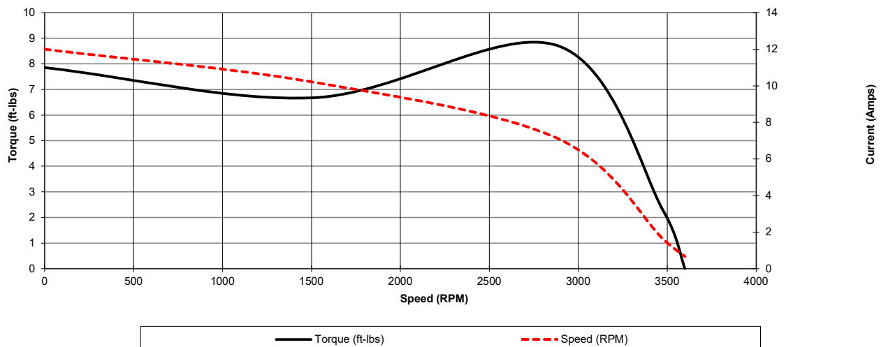
443T 484T Dual Voltage DOL 61 leads WYE Connection
